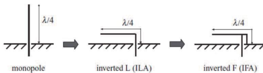
Figure.2. Inverted-F and Inverted-L antenna the reformed version of monopole
