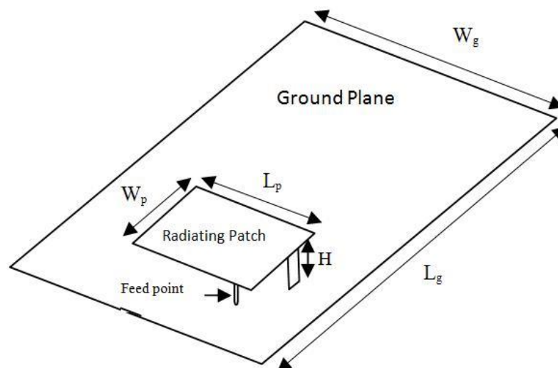
Figure.3. Structure of typical PIFA
